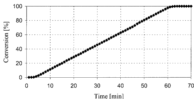
Figure 2. Hydrogen consumption in the asymmetric hydrogenation of 5 in 1,2-dichloroethane (1 bar \text{H}_2 pressure, catalyst 0.1 mol % [\text{Rh}(\text{COD})(\text{L2})_2]\text{BF}_4 , c(\text{5}) = 0.1 \text{ mol L}^{-1} )
