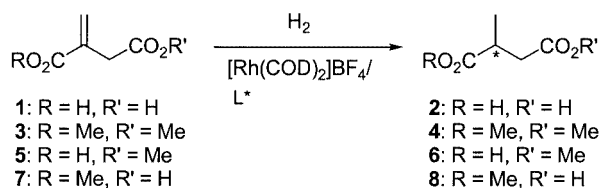
Scheme 3. Asymmetric hydrogenation of 2-methylenesuccinic acid and its derivatives. \text{L}^* = chiral phosphite ligand, COD = cyclooctadiene
